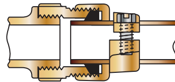
Pack Joint compression coupling for copper size tubing, P.E. pipe or PVC pipe
