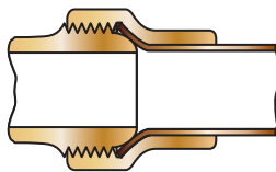
Flare Joint for connection to copper tubing
