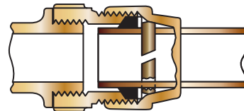
Grip Joint compression coupling for copper size tubing or P.E. pipe
