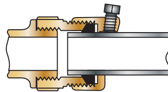
Pack Joint compression coupling for iron pipe
