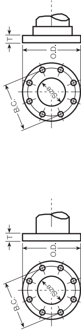
Threaded-On Flange ANSI/AWWA C115/A21.15
