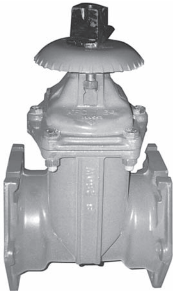
Valve shown with Gate Box Aligner installed under operating nut
