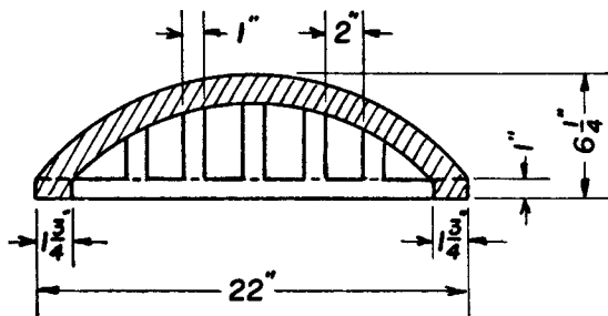
R-4351-D Beehive Grate
