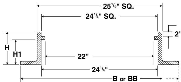
Details of grate indicate water flow is from left to right
