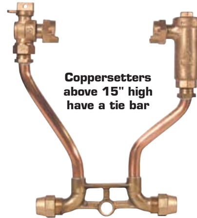
70 Series Coppersetter shown with Angle Ball Valve on inlet and Cartridge Dual Check Valve on outlet. Also with Brace Pipe Eye.
